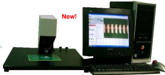
Solder Paste Height Checker
