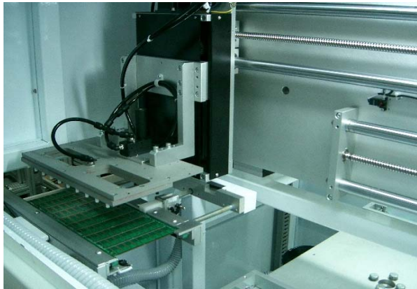
Front of machine where the board is positioned, picked up and transferred.
