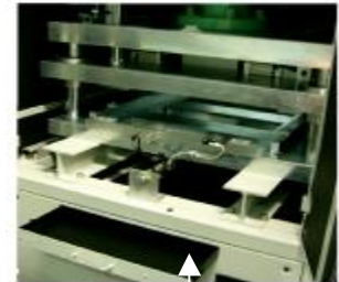
Tray collection and removals of slugs.
